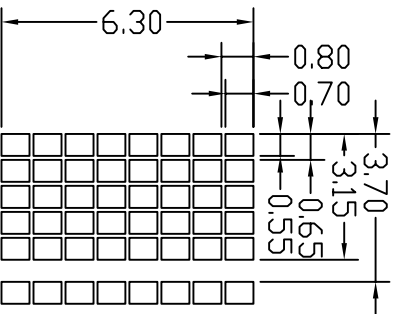
DOT SIZE SCALE 4:1
